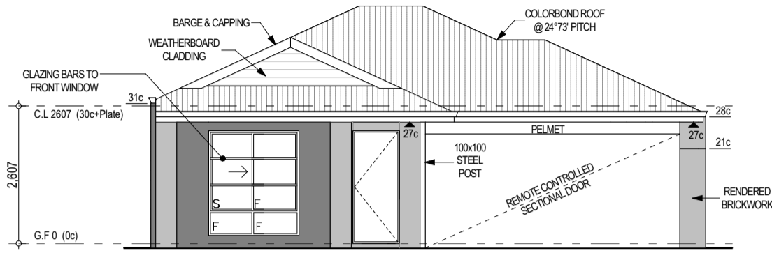
1 FRONT ELEVATION 1:100
